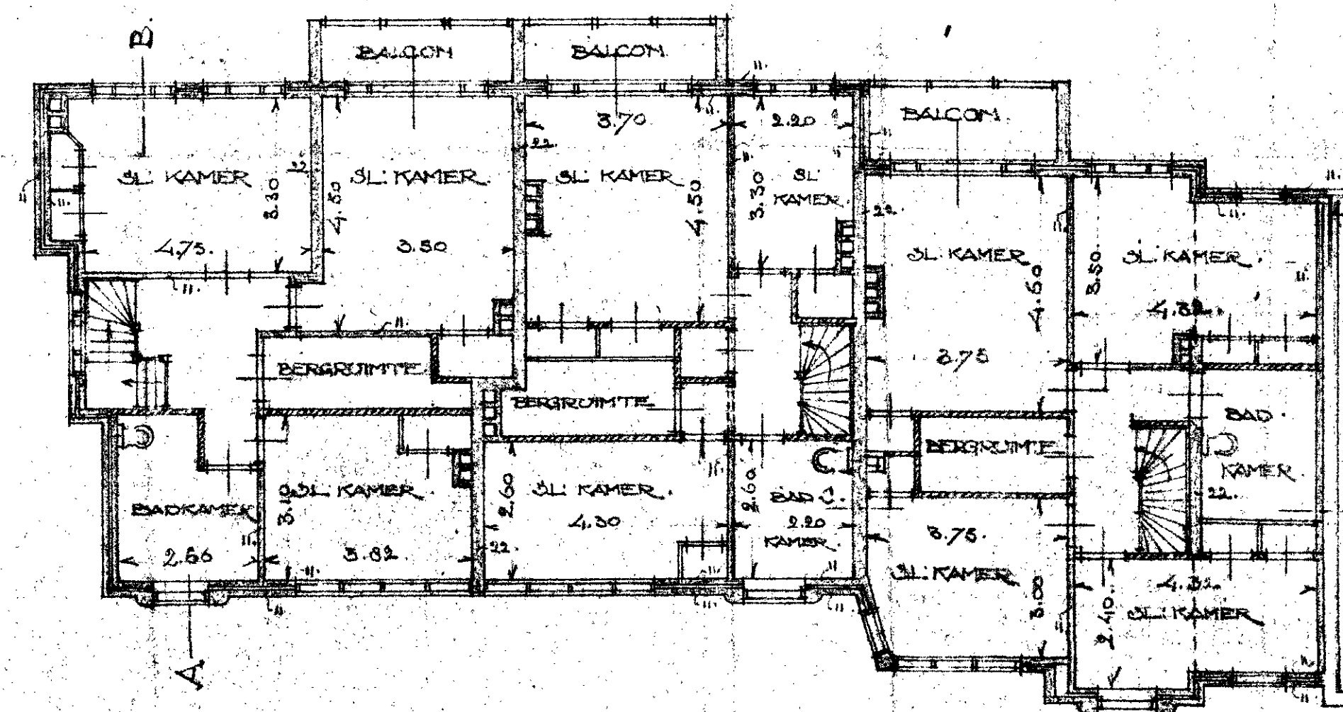
VERDIEPING.
