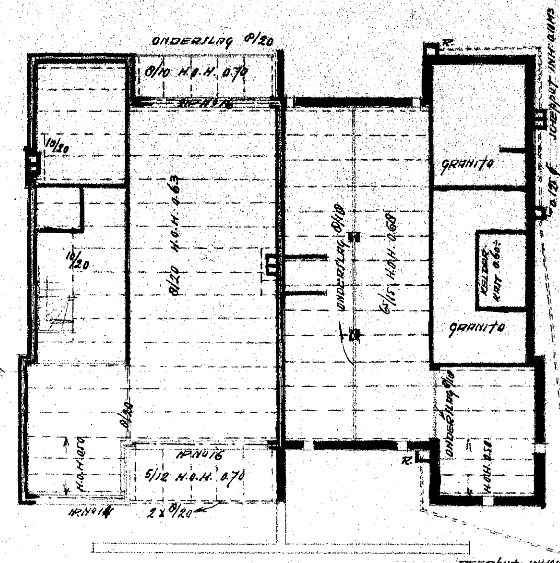
PLAN BEGANE GROND
