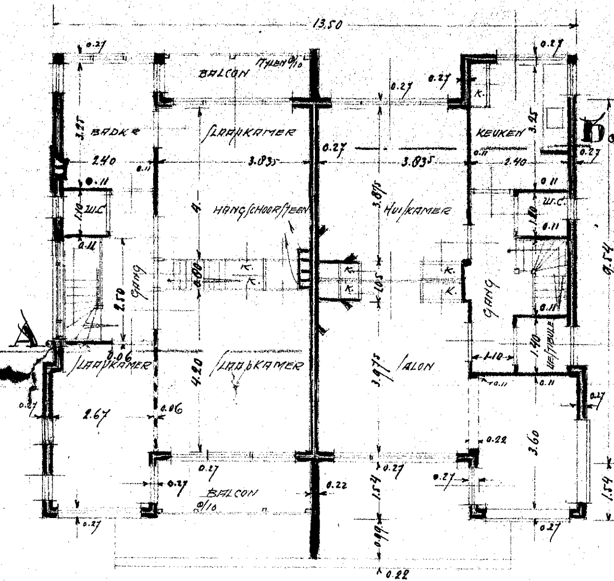
PLAN VERDIEPING
