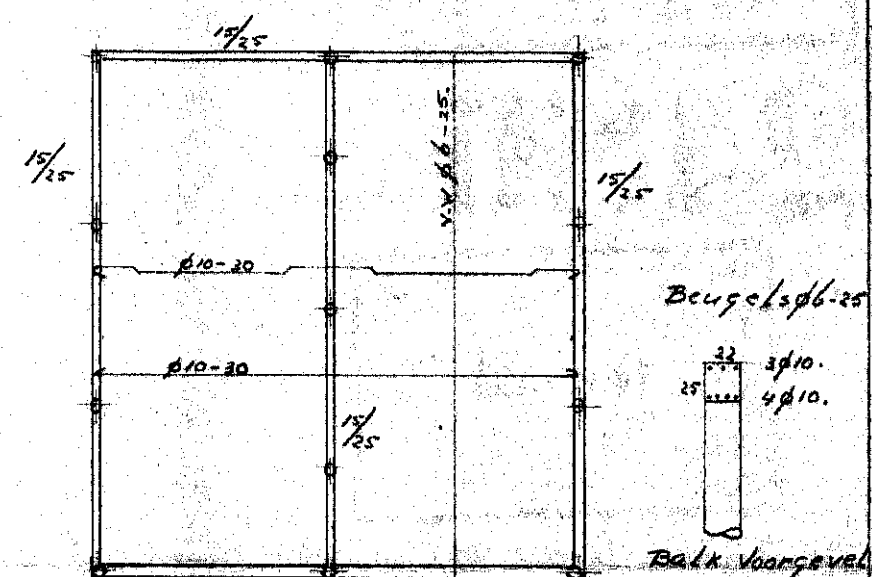
12/25. Platte grond betonfundering.
