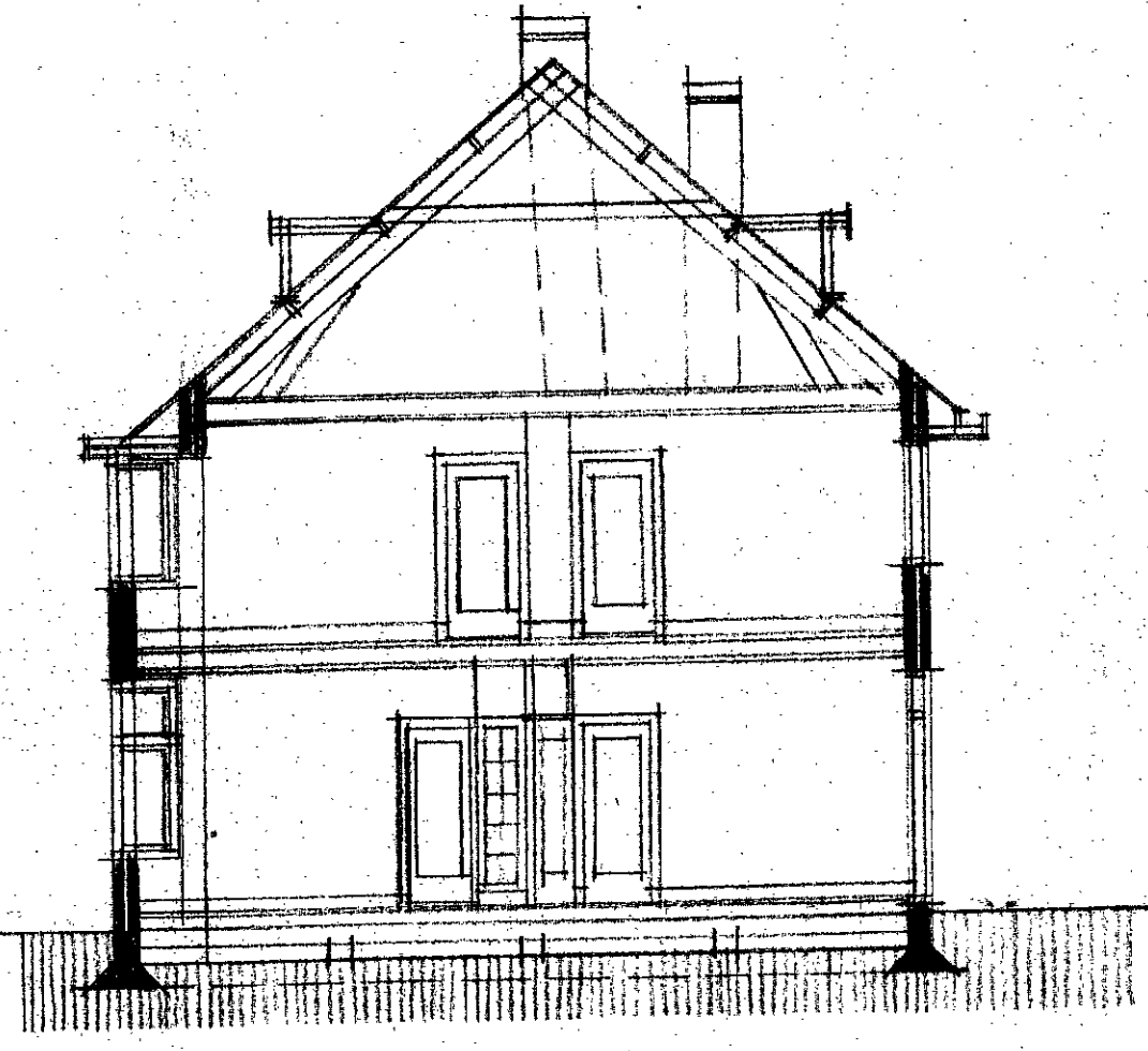
© DOORSNEDE CD ©
