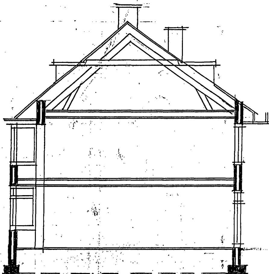
DOORSNED
