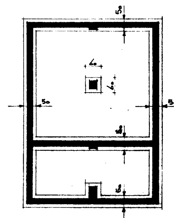
.fundering.
